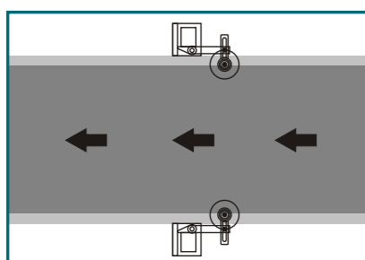
自动输送防偏保护装置 Protective device against side running of conveyor belt
